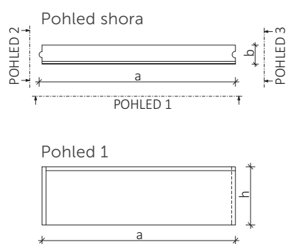
B&BC ABO 5-15
