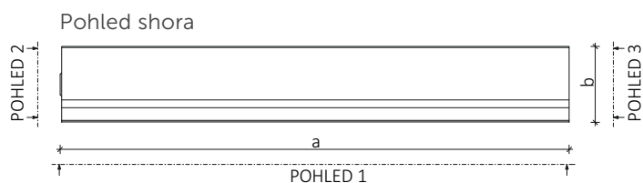
B&amp;BC ABO 15-30
