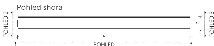
B&BC ABO 8-25
