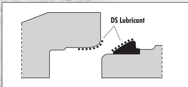
Example: slide seal in front of shoulder of spigot end
