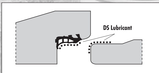
Example: integrated pipe seal
